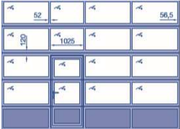
Version with wicket door and threshold rail
