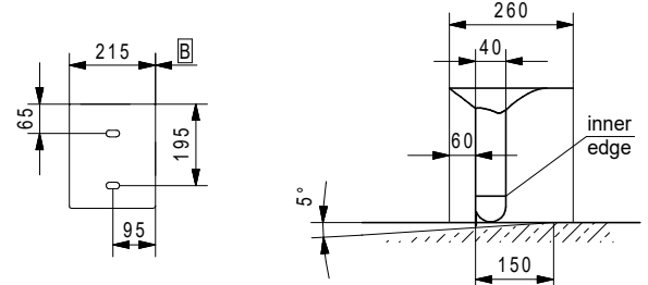
Detail Y: fixing points for ground plate 2 points fixing hole 15 x 30
