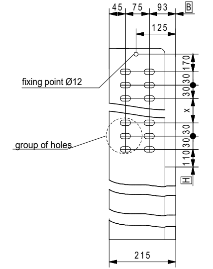
Detail X: fixing points for frame top part as well as 1 per each group of holes, fixing hole 15 x 30
