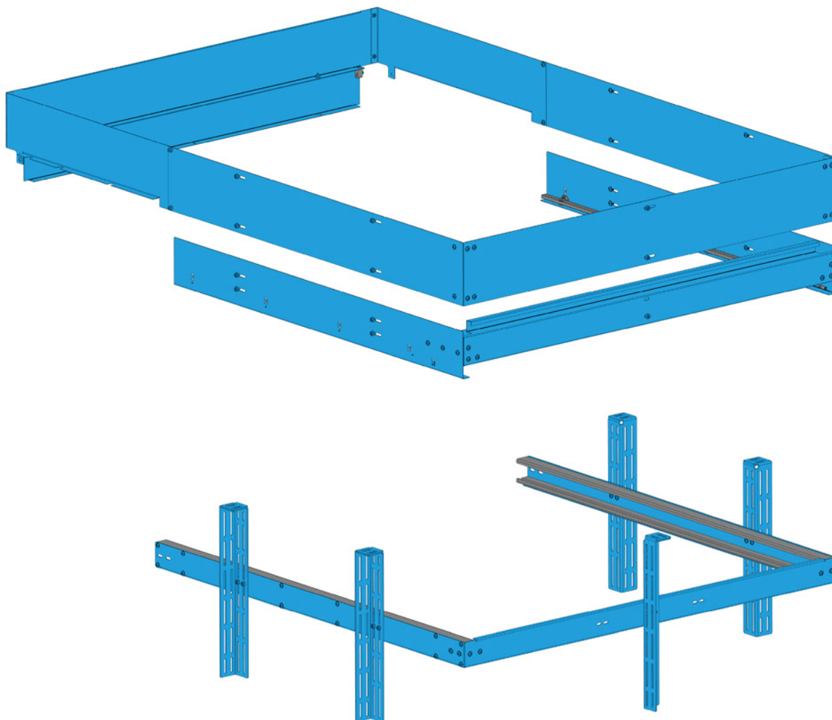
Fig. 73: Spiral case
