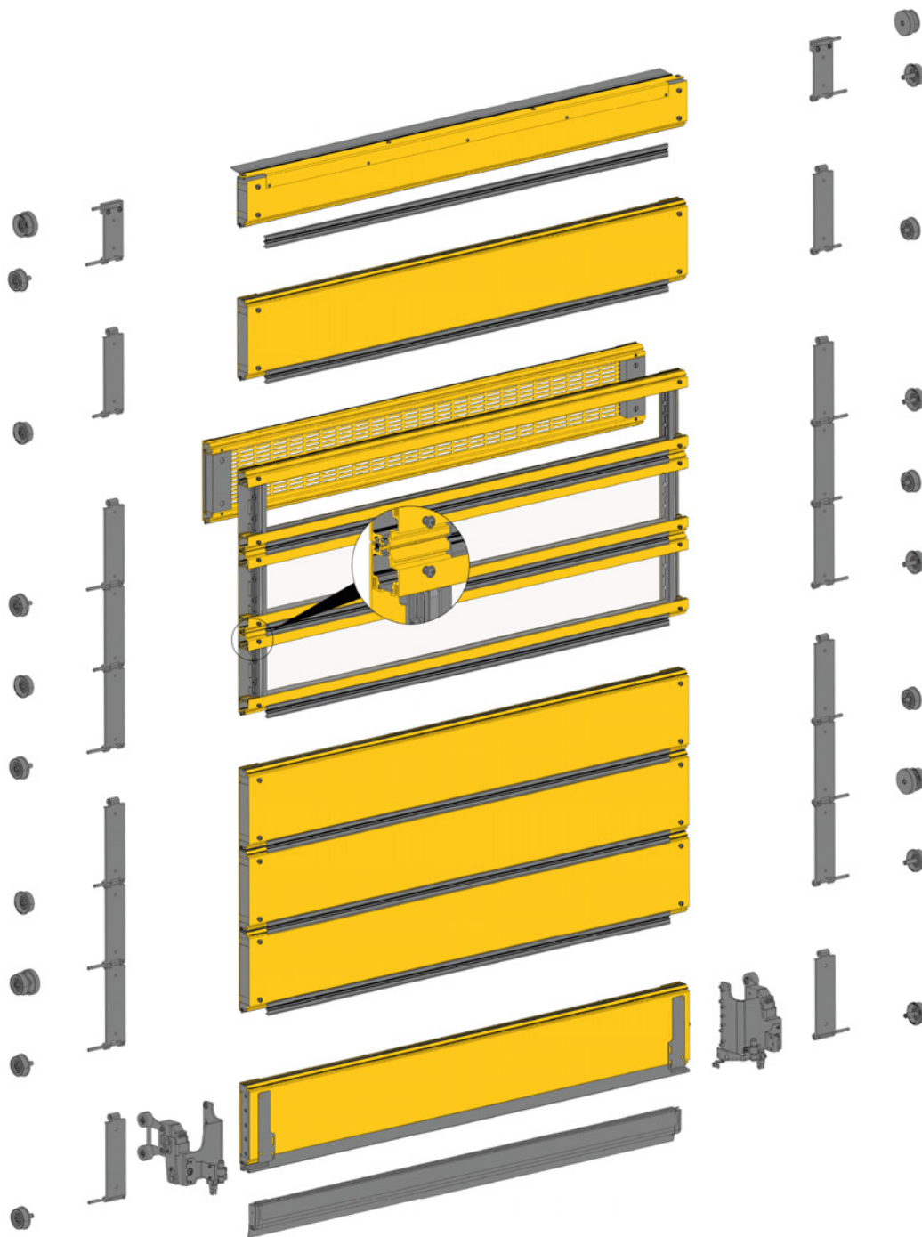
Fig. 67: Coating for door leaf
