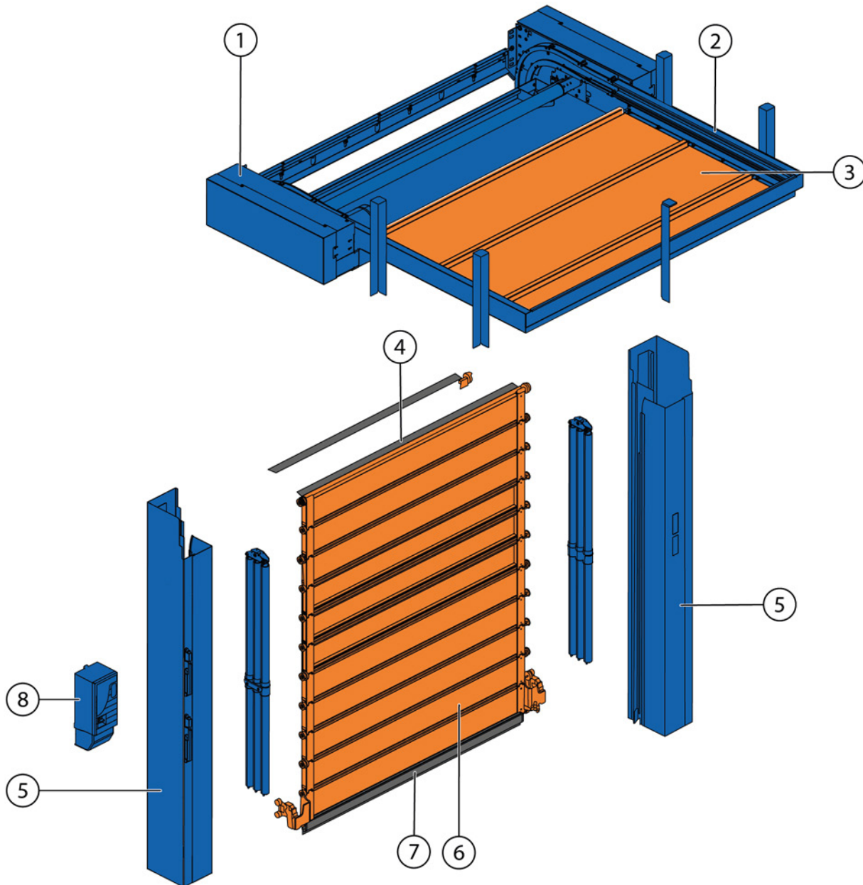
Fig. 4: Assemblies
