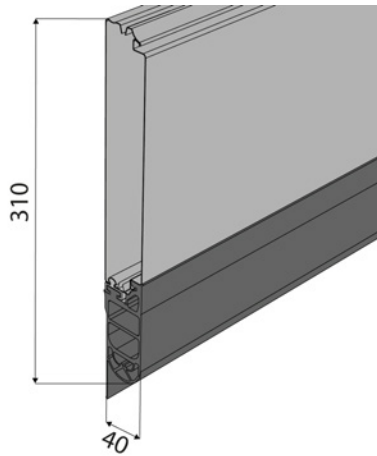
Fig. 45: Closing strip
