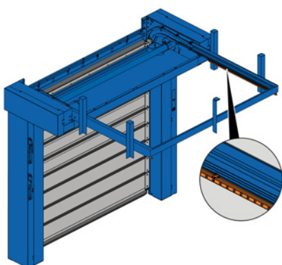
Fig. 10: Protective guard with door light grid (optional)
