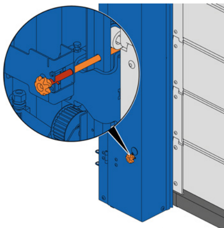
Fig. 23: Door leaf locking with bolt
