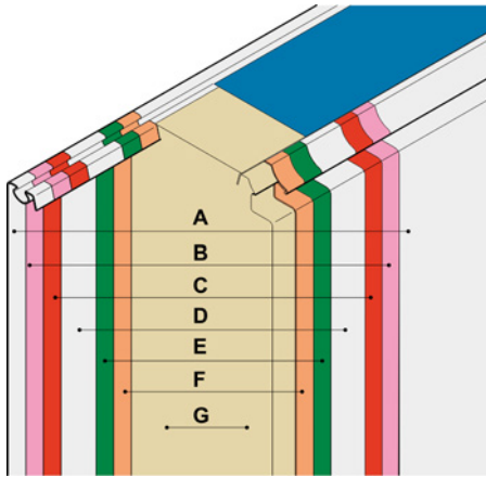
Fig. 42: Structure of the EFA-THERM® lath
