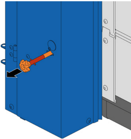
Fig. 25: Door leaf locking with bolt, unlocked
