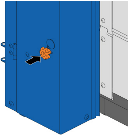
Fig. 24: Door leaf locking with bolt, locked
