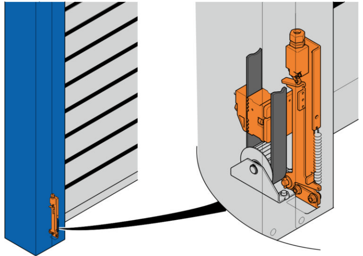
Fig. 10: Door locking mechanism
