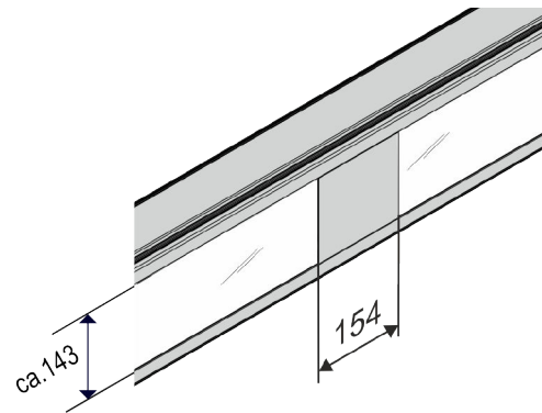
Fig. 32: Width, middle bar
