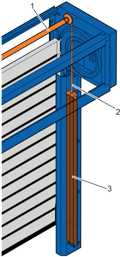
Fig. 20: Counterbalance
