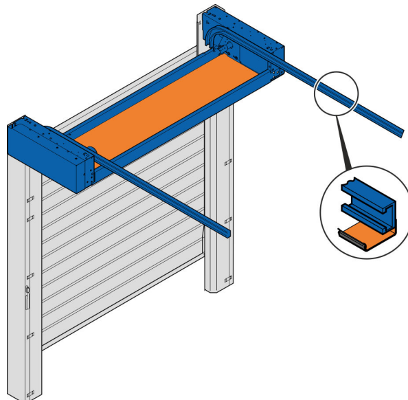
Fig. 16: Low lintel spiral case cover
