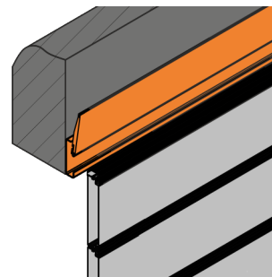
Fig. 44: Sealing profile open
