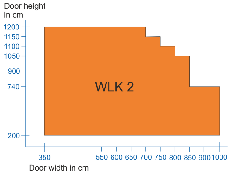
Fig. 8: Diagram, wind load class (WLC) 2 for door system type 305
