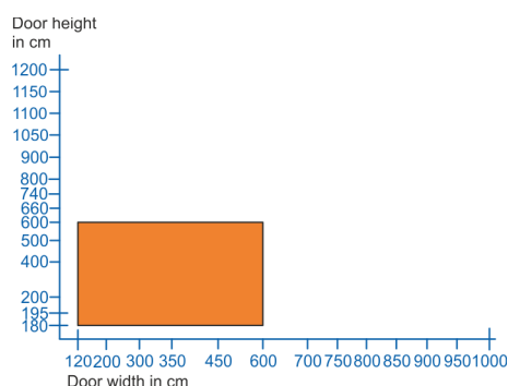
Fig. 4: Diagram of possible door system heights and door system widths
