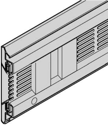
Fig. 31: EFA-VENT ventilation lath
