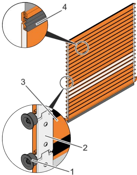
Fig. 26: Door leaf with 20 mm thick EFA-ALUX aluminium laths and a spacing of 151 mm (AST)
