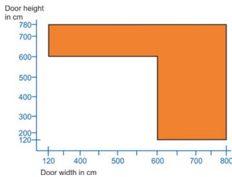
Fig. 11: Diagram of possible door system heights and door system widths
