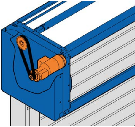
Fig. 33: Drive, door system types 237 R; 237 O; 243 N; 238 R; 238 O; 236 N; 231 R; 272 N; 232 R
