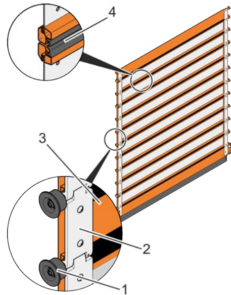
Fig. 27: Door leaf with 30 mm thick EFA-CLEAR sight laths and a spacing of 225 mm (LKZ)
