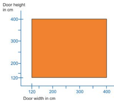
Fig. 10: Diagram of possible door system heights and door system widths
