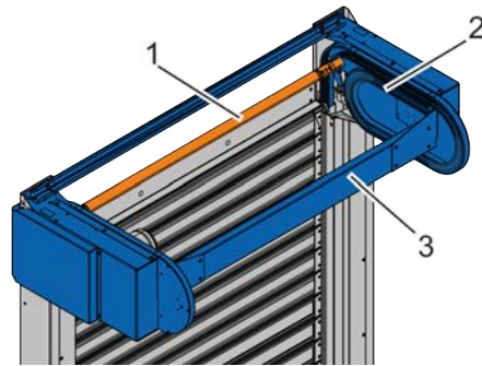
Fig. 15: Oval spiral case
