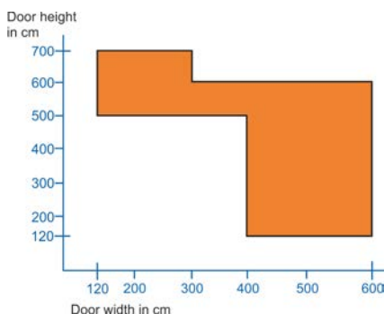
Fig. 9: Diagram of possible door system heights and door system widths
