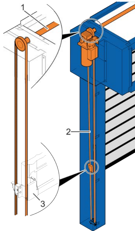
Fig. 21: Round and oval spiral transmission of force
