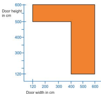
Fig. 4: Diagram of possible door system heights and door system widths
