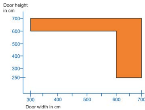
Fig. 6: Diagram of possible door system heights and door system widths
