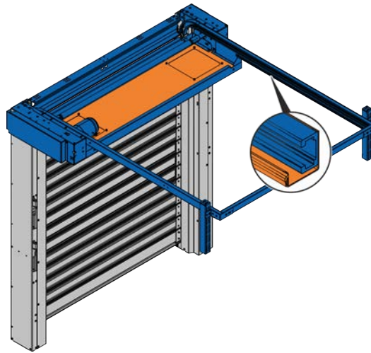
Fig. 18: Low lintel spiral case cover
